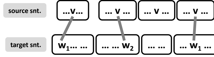
Figure 4: Feature of f_{doc}^{st} . A source-side word v appears four times and is translated three times to two different target-side words w_1 and w_2 . For v , we have a ratio of \log \frac{3}{2} .
